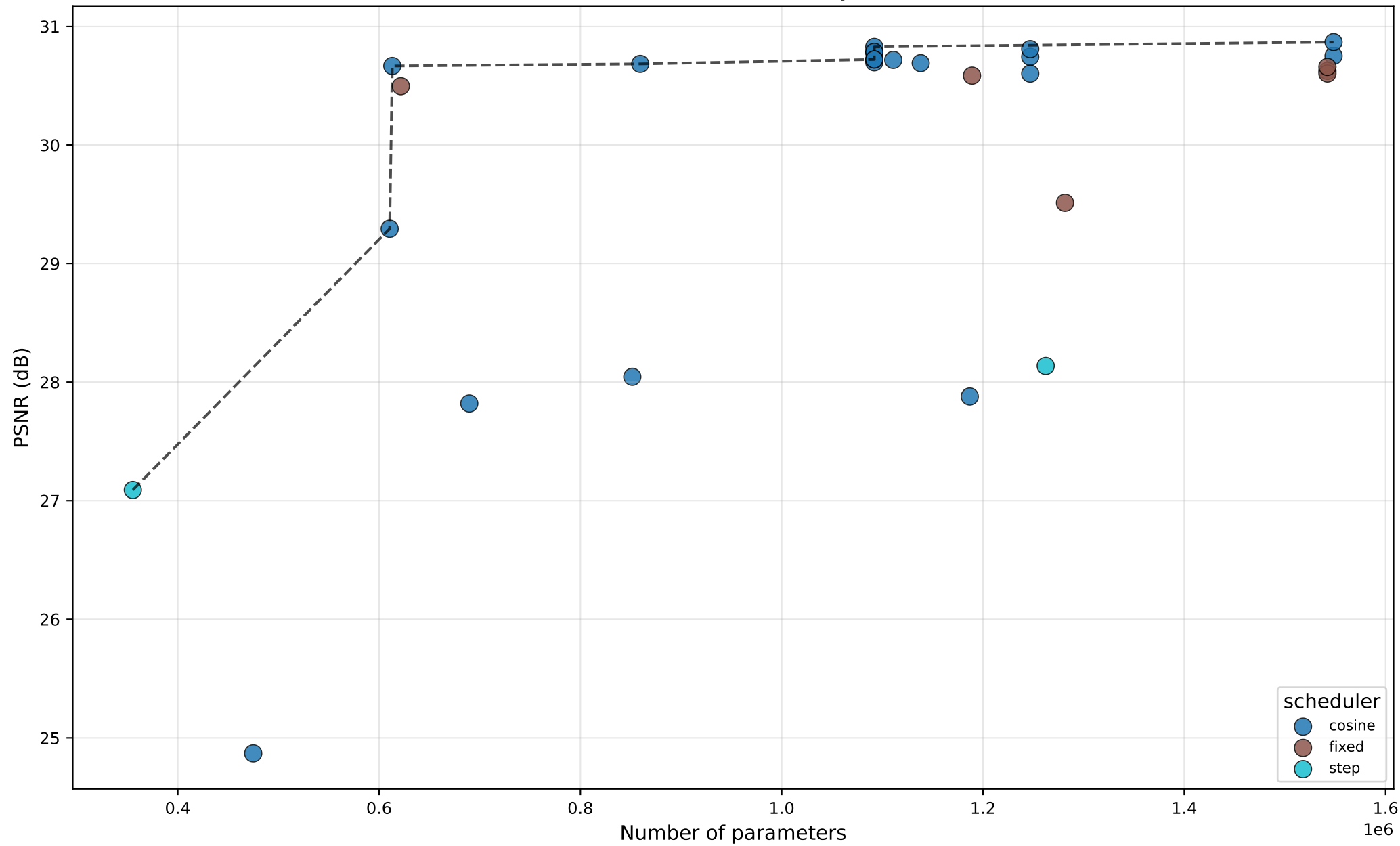
PSNR vs #Params — HAT — by scheduler
